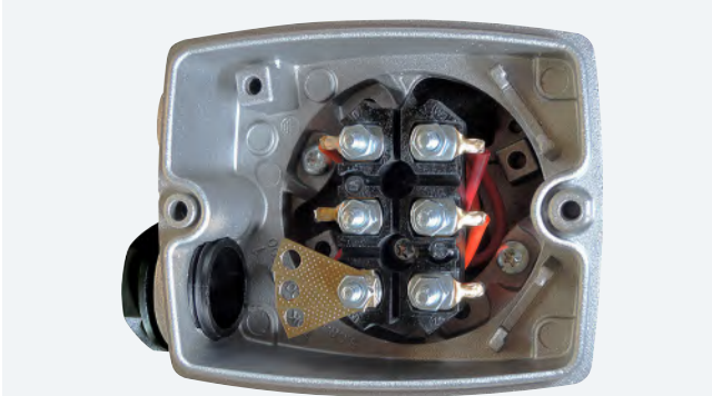
Terminal box types TB1F00, TB1H00, TB1J00
