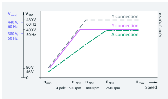
Operating characteristics of Innomotics GP/SD VSD4000 line motors 1)
