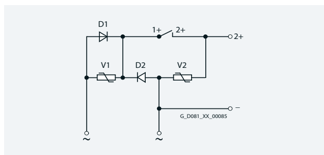
Half-wave rectifier 400 V AC
